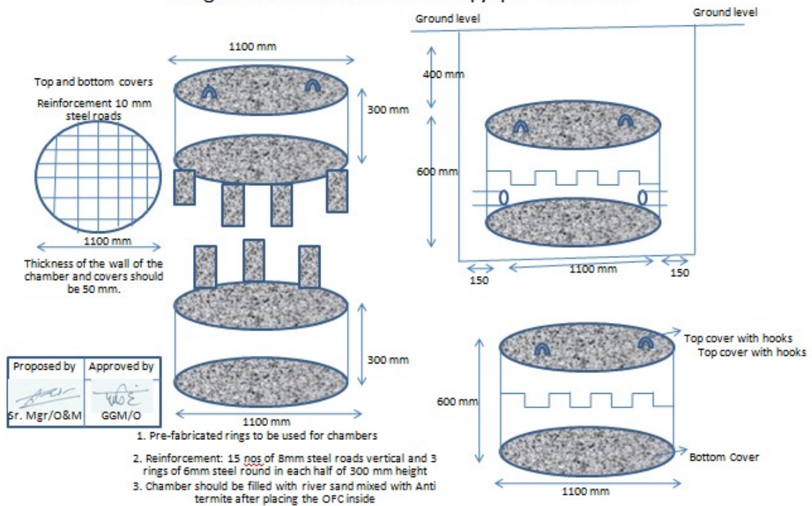
Diagram of construction of loop/splice chamber
