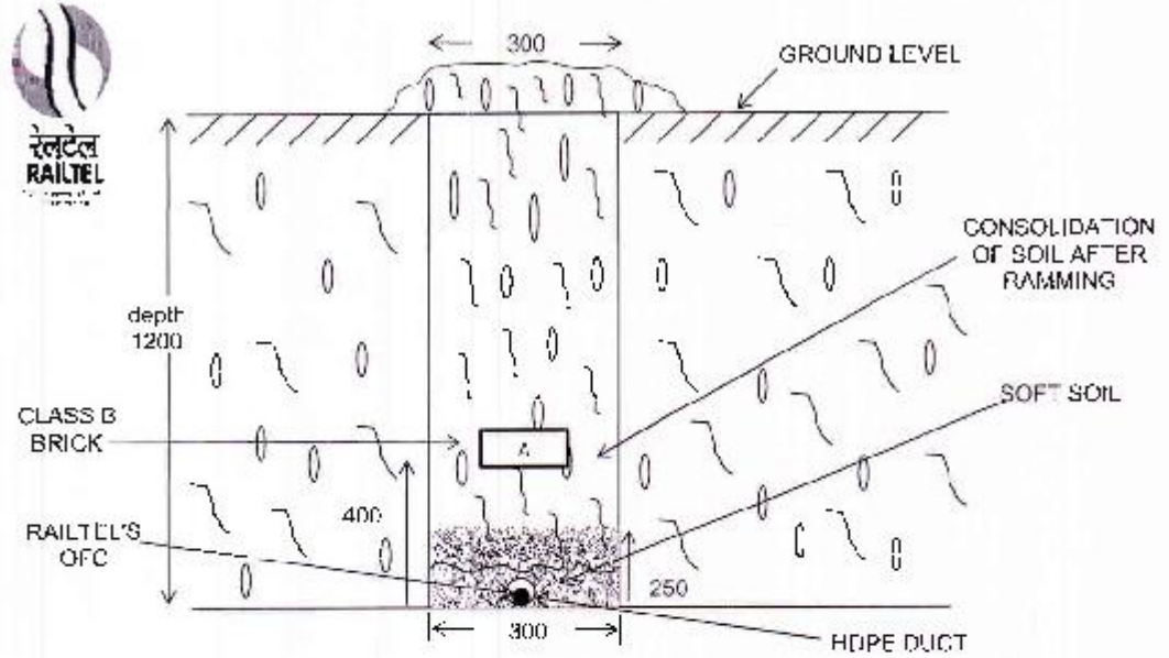
(TRENCHING IN NON ROCKY SOIL) ALL MENTIONED DIMENSIONS ARE IN MILIMETER
