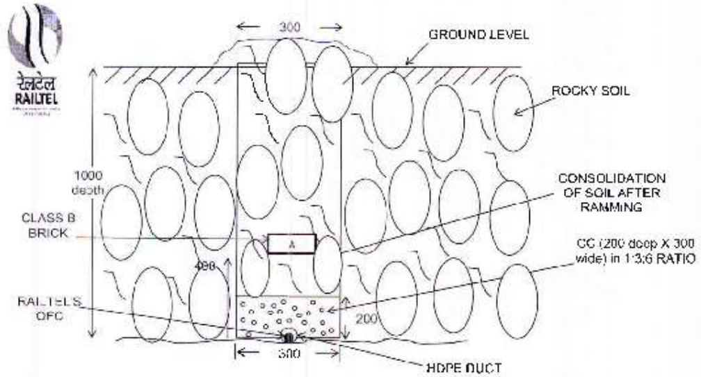
(TRENCHING IN ROCKY SOIL) ALL MENTIONED DIMENSIONS ARE IN MILLIMETER
