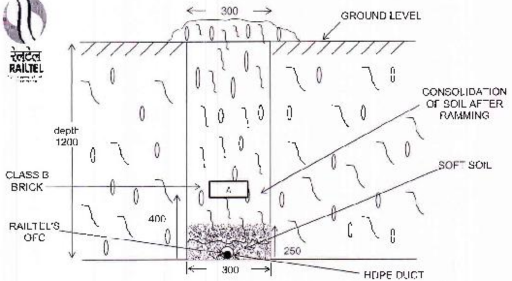
(TRENCHING IN NON ROCKY SOIL) ALL MENTIONED DIMENSIONS ARE IN MILLIMETER
