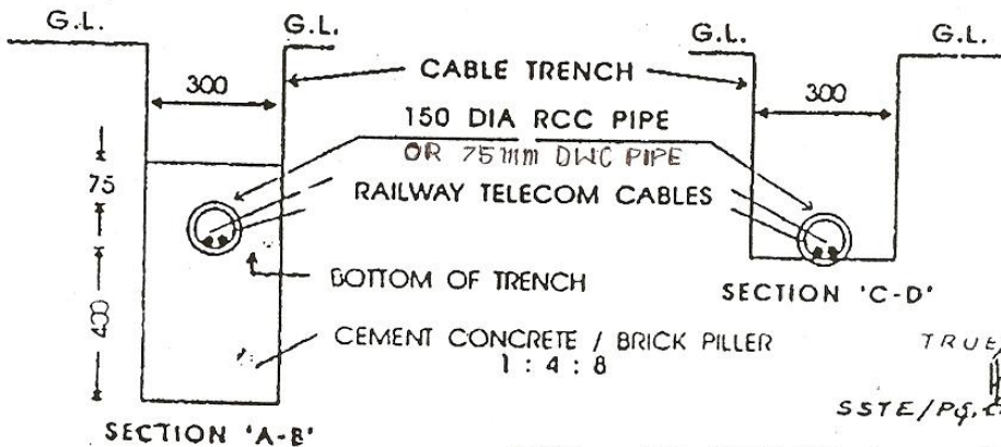
SECTION 'A-B'
