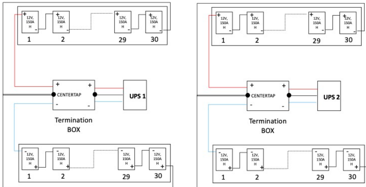
Connectivity Configuration of Existing UPS Battery Setup
