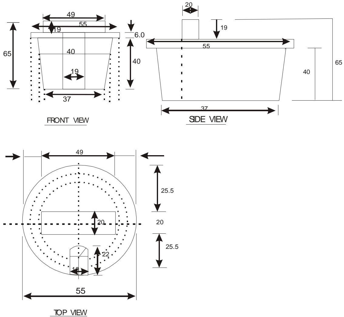
Figure 2 Rubber Cork
