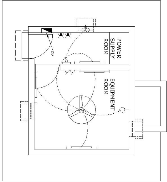
SMALL ROOM (ELECTRICAL LAYOUT PLAN)
