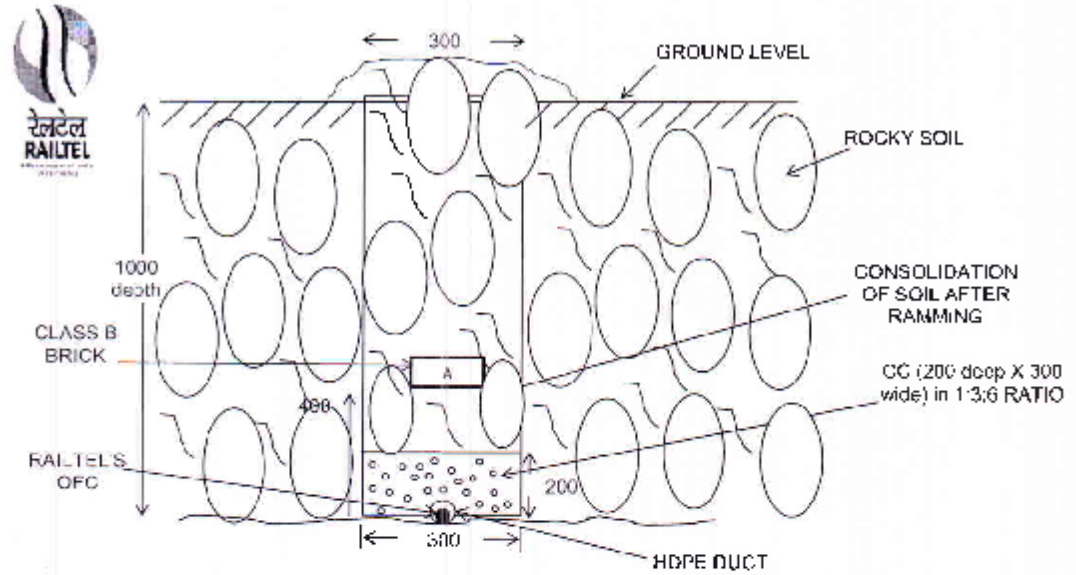
(TRENCHING IN ROCKY SOIL) ALL MENTIONED DIMENSIONS ARE IN MILIMETER
