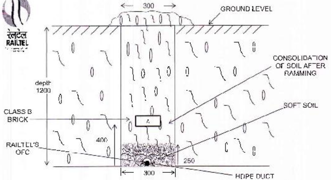
(TRENCHING IN NON ROCKY SOIL) ALL MENTIONED DIMENSIONS ARE IN MILIMETER
