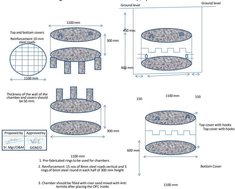
Diagram of construction of loop/splice chamber
